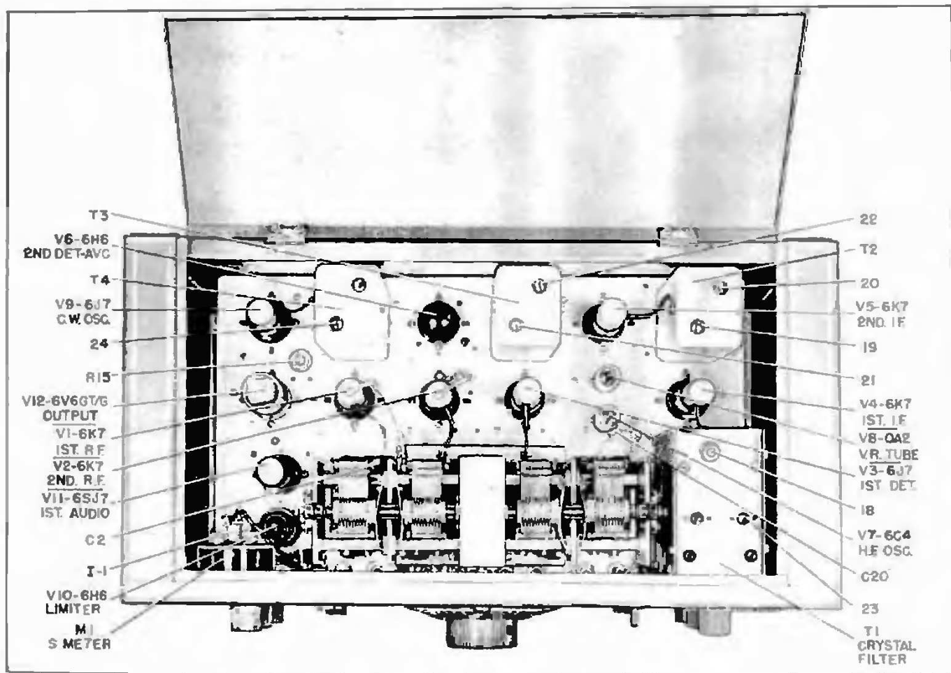
Figure No. 5. Top View of Receiver
