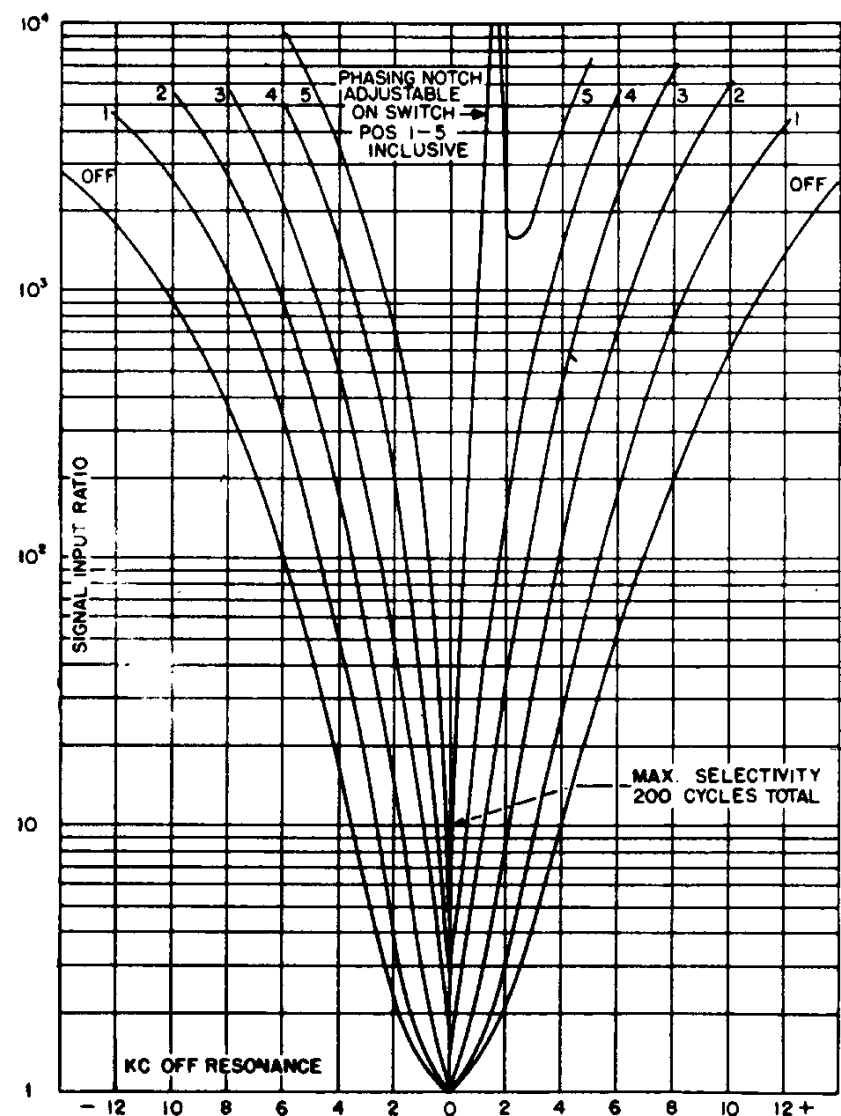
Figure No. 1. Crystal Filter Selectivity Curves.
