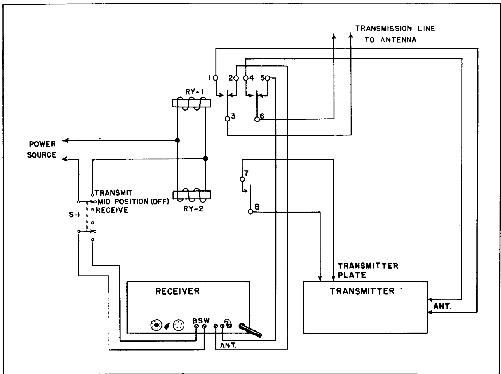
Figure No. 3. Typical Antenna Switching System
