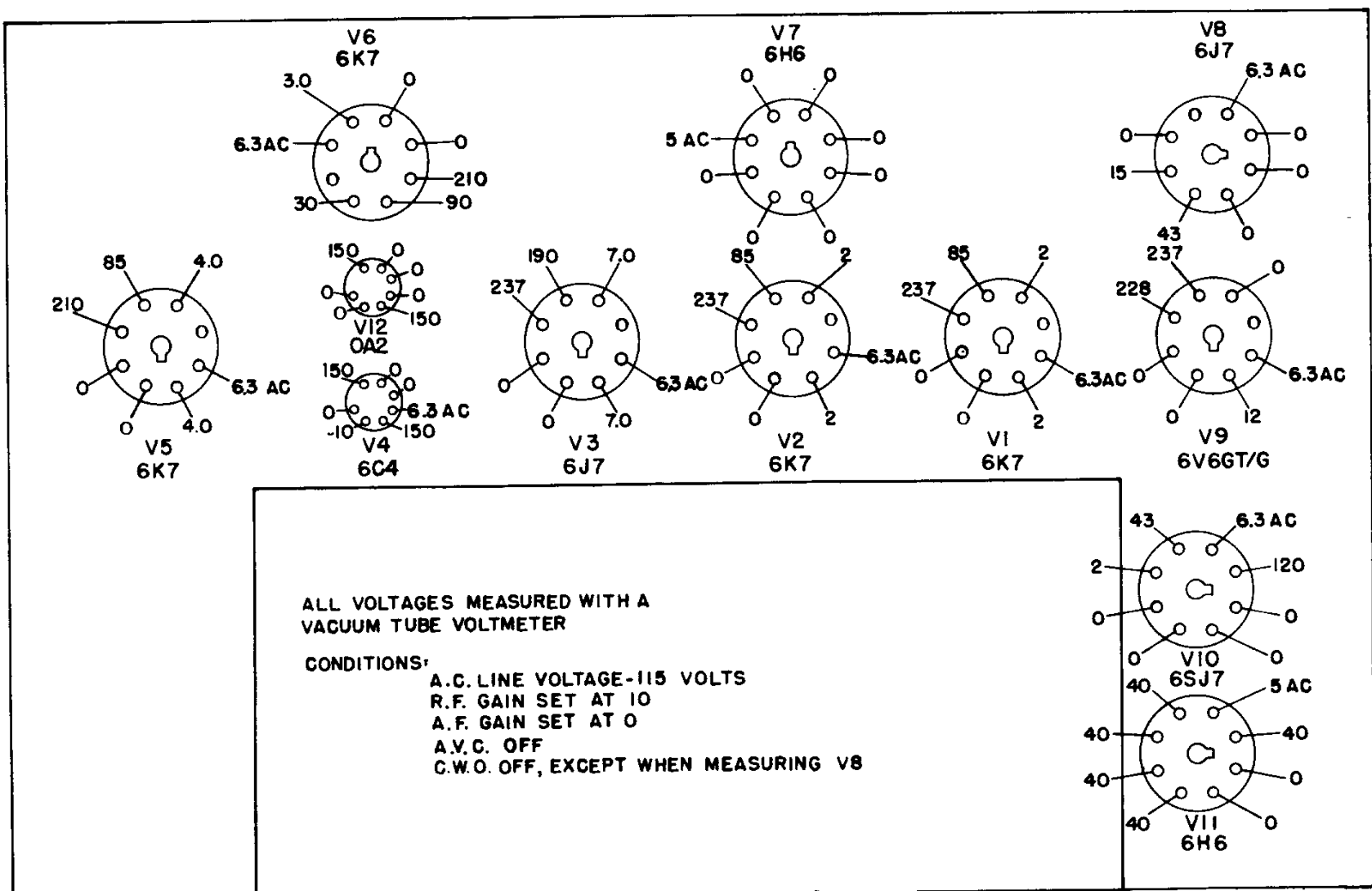
Figure No. 7. Tube Socket Voltages
